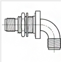
90° sweep SMA jack - SMA jack, bulkhead Part no. 29525
