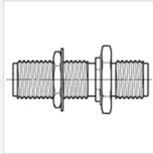
SMA jack - SMA jack, bulkhead Part no. 29041-3
