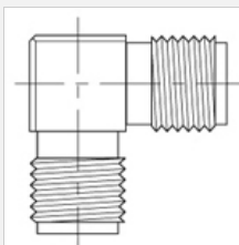
Right angle SMA jack - SMA jack Part no. 29212-3
