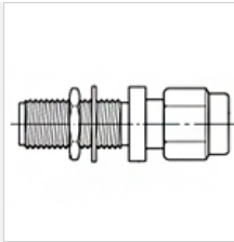
SMA jack - SMA plug, bulkhead Part no. 29089-2
