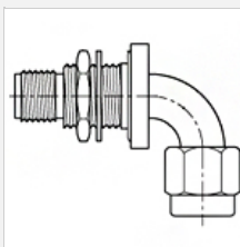
90° sweep SMA jack - SMA plug, bulkhead Part no. 29526
