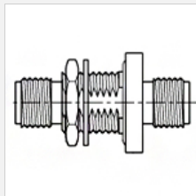
SMA jack - SMA jack, bulkhead Part no. 29285G
