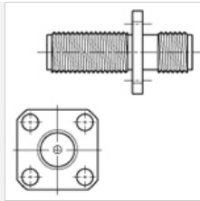
SMA jack - SMA jack, flanged Part no. 29074F-1
