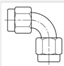
90° sweep SMA plug - SMA plug Part no. 29519
