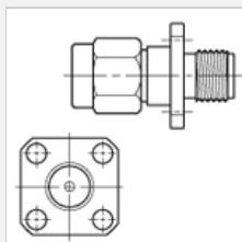
SMA plug - SMA jack, flanged Part no. 29089F
