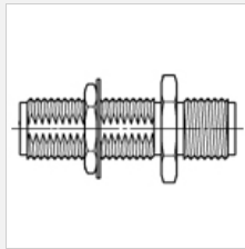
SMA jack - SMA jack, bulkhead Part no. 29041-1
