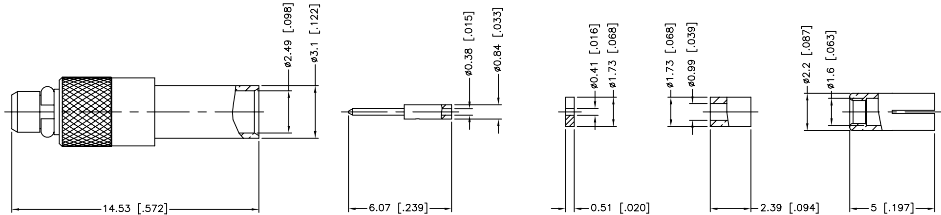
RECOMMENDED CABLE STRIPPING DIM'S
