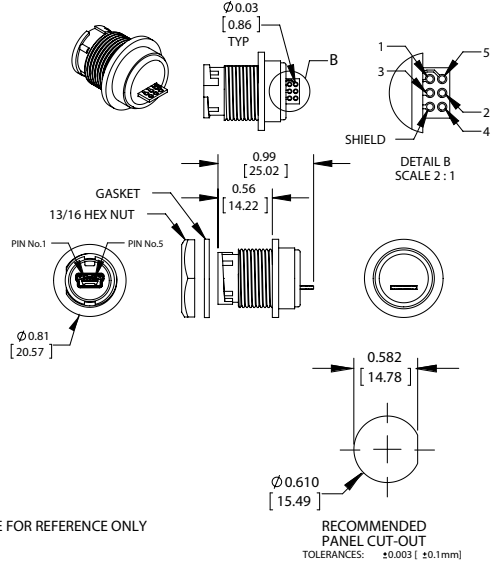
DCP-USBNB-MNSC USB Mini-B to Solder Holes
