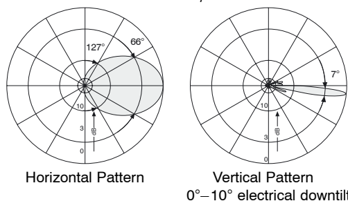
1850 – 1990 MHz: +45°/–45° Polarization
