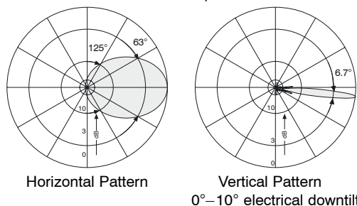
1920 – 2170 MHz: +45°/–45° Polarization
