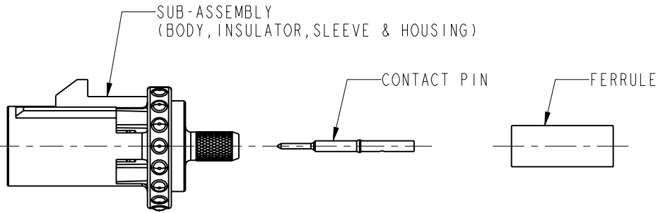
TYPICAL CONNECTOR COMPONENTS [ SHOWN AS 2FA16NXSP-C01-1 CONFIGURATION ]
