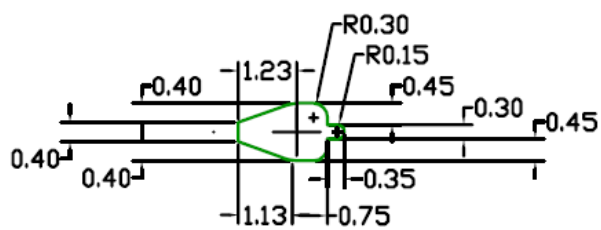
Soldermask
