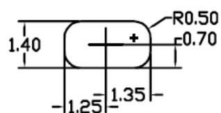
Footprint and Pastemask
