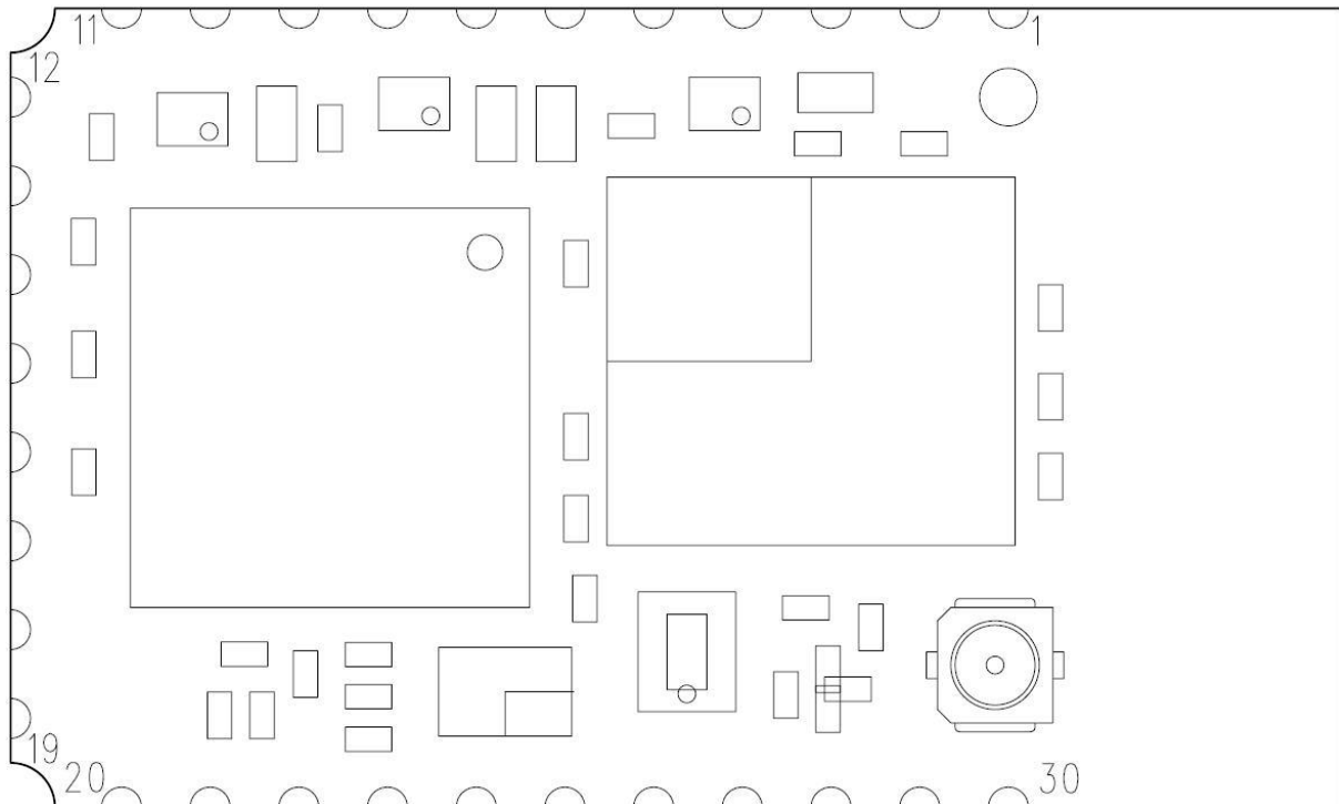
Figure 1: RTX4140 pin numbering
