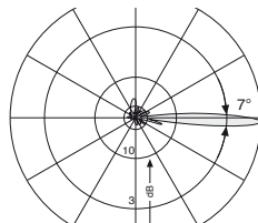
Vertical Pattern 0°–8° electrical downtilt
