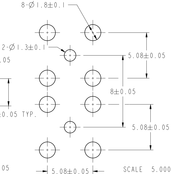
RECOMMENDED PCB LAYOUT DIMENSIONS
