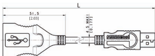
Part Number : USBAP 6 xxxA WITH USB-A PLUG
