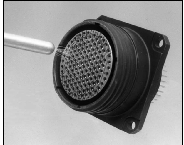
ESD Testing on MIL-DTL-38999, Series III Filter Cylindrical Connector (Actual Photo)
