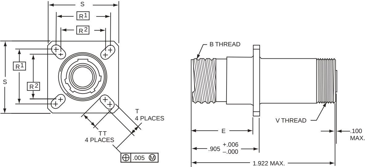
21-50X0XX-XXX UTS (Crimp) Contact MIL-C-39029/57
