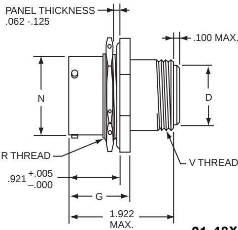
21-48X7XX-XXX UTS (Crimp) Contact MIL-C-39029/57
