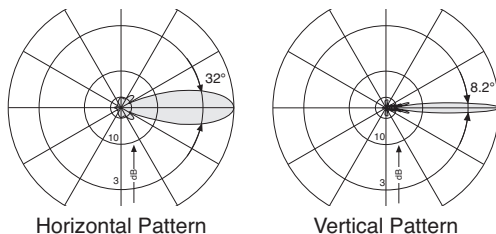
824 – 894 MHz: +45°/–45° Polarization
