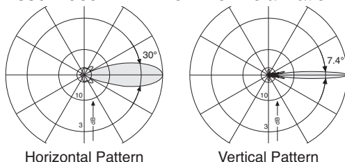
880 – 960 MHz: +45°/–45° Polarization
