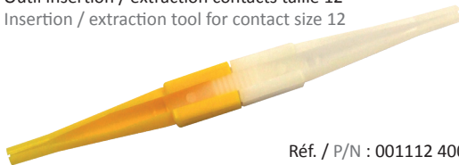
Outil insertion / extraction contacts taille 12 Insertion / extraction tool for contact size 12
