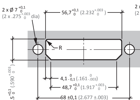
Perçage standard Standard cutout
