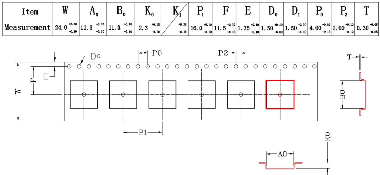
Figure 10. CYBLE-214015-01 Tape Dimensions
