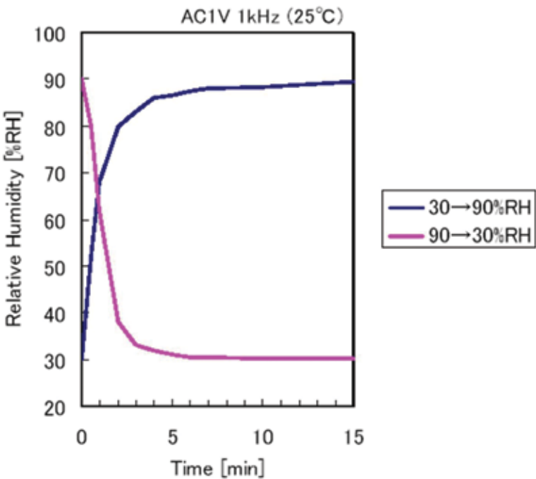
Figure 2 : Typical Response
