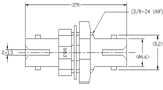
ST Metal Adapter, Feed-through, D-Hole
