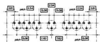
F032/M032 contacts
