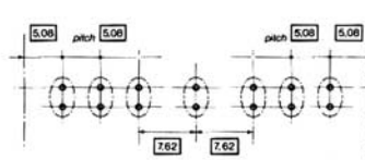
F041/M041 contacts
