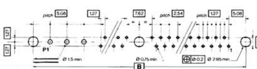
⑧ Mother board
