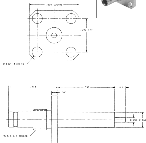
Straight 4-Hole Flange 102-233-01 102-233-10 102-233-20 102-233-30
