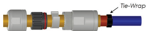
Step 3: Cut tie wrap to remove excessive material. Trim shielding flush to edge of tie wrap
