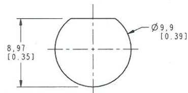
SCALE 3.000 MOUNTING HOLE DETAIL MAX PANEL THK. 104
