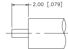
RECOMMENDED CABLE STRIPPING DIMENSIONS
