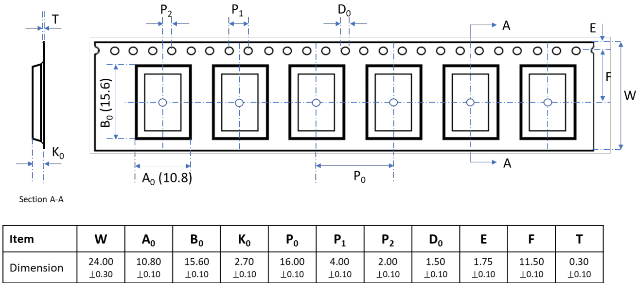
Figure 12. SGW1010/SGW1011 Tape Dimensions
