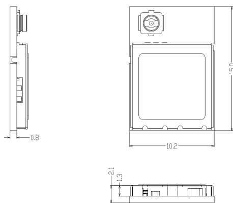
Figure 8. SGW1011 (External Antenna) Mechanical Information
