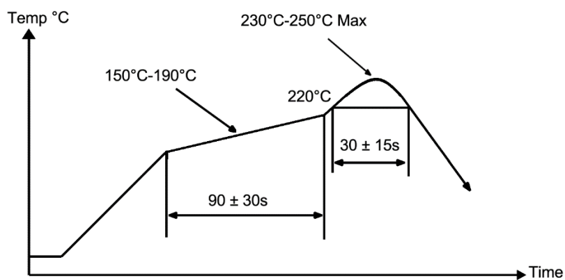
Figure 11. Soldering Temperature-Time Profile for Re-Flow Soldering
