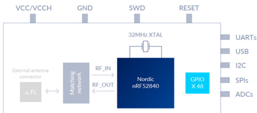
Figure 2. SGW1011 (External Antenna) Block Diagram
