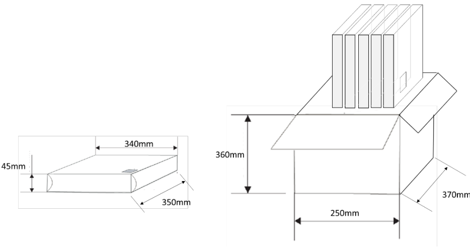
Figure 13. SGW1010/SGW1011 Reel Packaging
