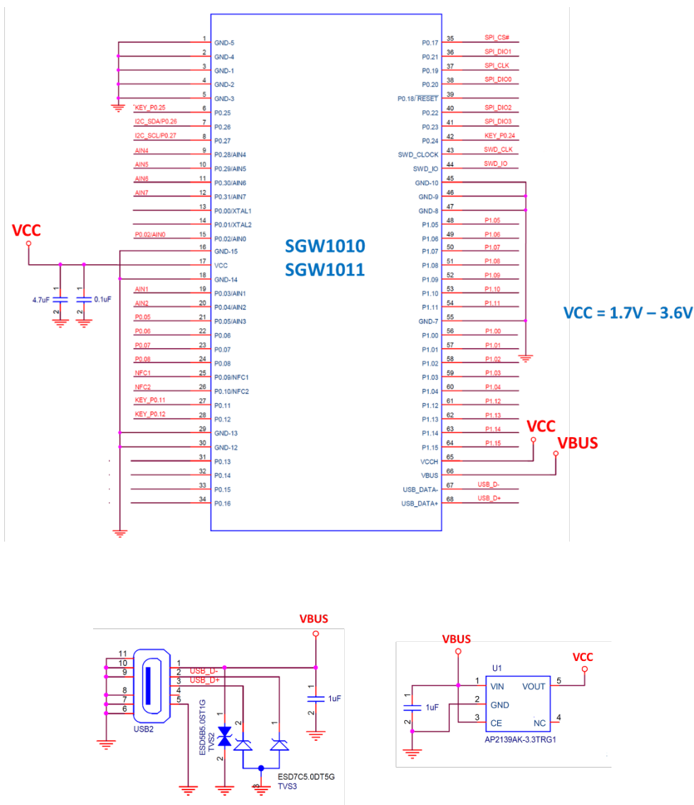
Figure 4. SGW1010/SGW1011 Low Voltage Mode Application Example
