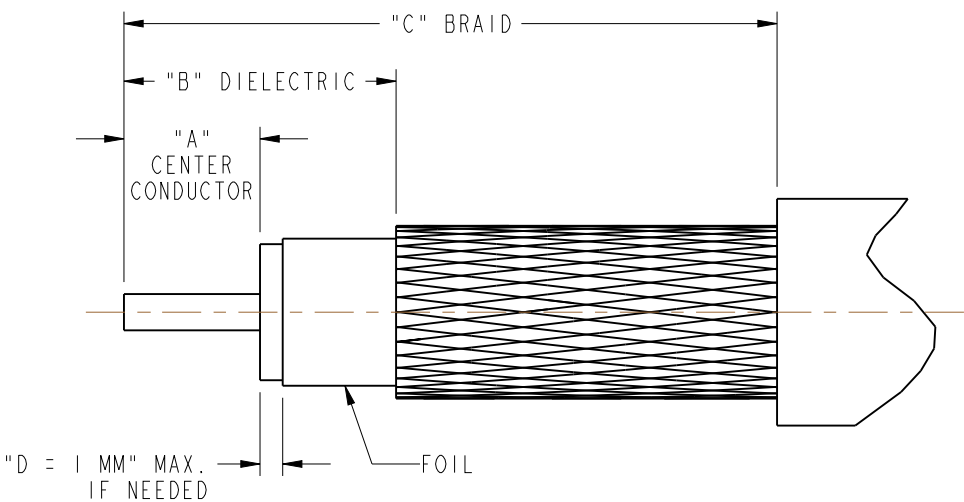
RECOMMENDED CABLE STRIPPING DIMENSIONS SCALE 6.000
