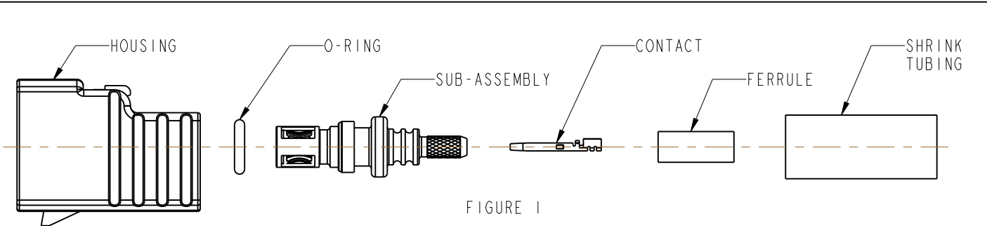
TYPICAL CONNECTOR COMPONENTS [ SHOWN AS 3FA1-NXSJ-C01E6 CONFIGURATION ]
