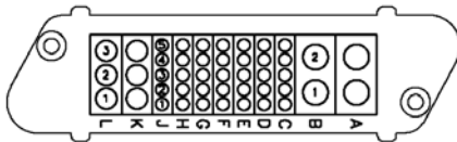
Plug Rep 37 and 237 Recept. Rep 137 and 337
