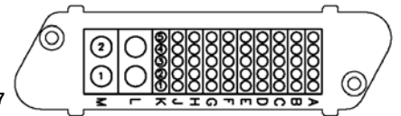
Plug Rep 47 and 247 Recept. Rep 147 and 347
