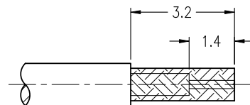
RECOMMENDED STRIPPING DIM'S
