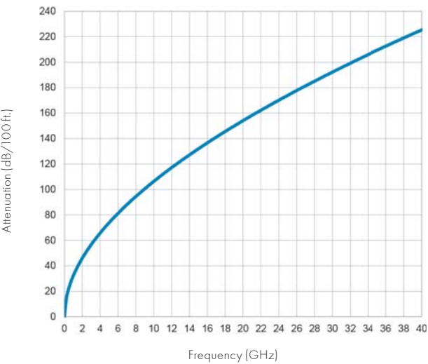
Graph 1: Cable attenuation
