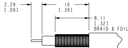
SUGGESTED CABLE TRIMMING DIMENSIONS
