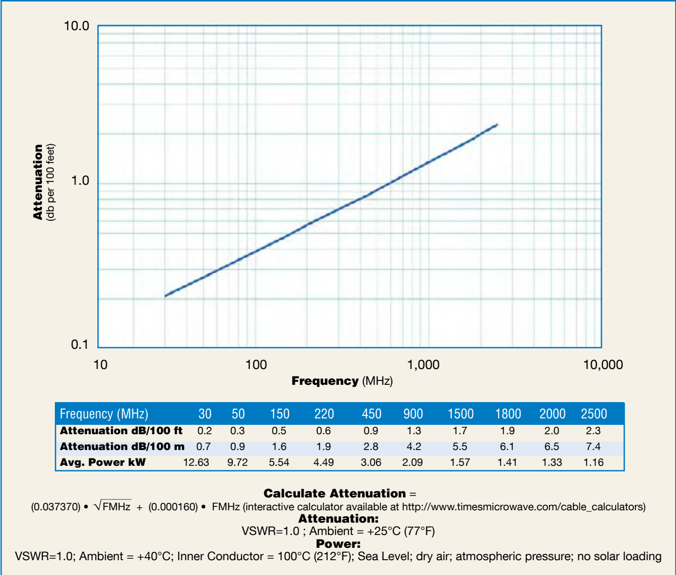
Attenuation vs. Frequency (typical)
