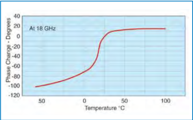
Fig. 10 Phase Stability
