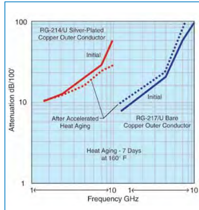
Fig. 5 Attenuation Stability
