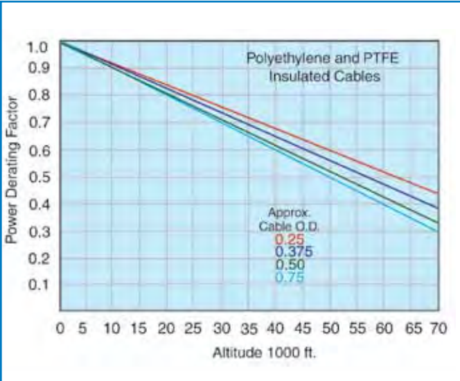
Fig. 7 Power Altitude Correction Factor
