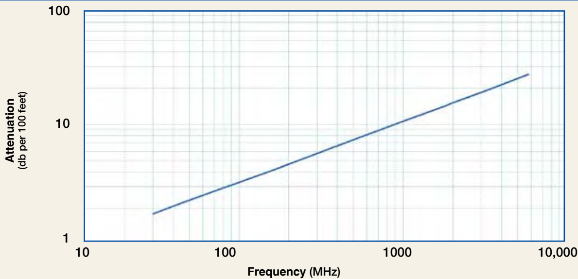
Attenuation vs. Frequency (typical)
