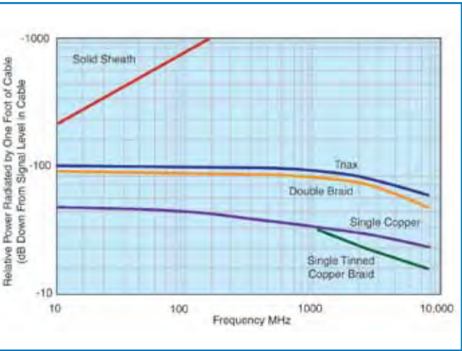
Fig. 9 Shielding Effectiveness
