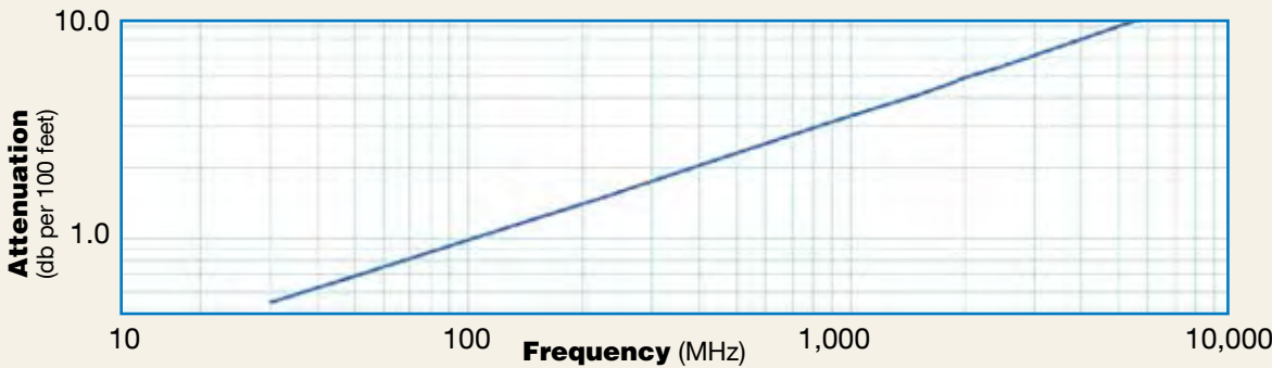
Attenuation vs. Frequency (typical)
