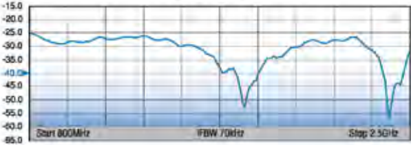
§11 TYPICAL RETURN LOSS(dB)
