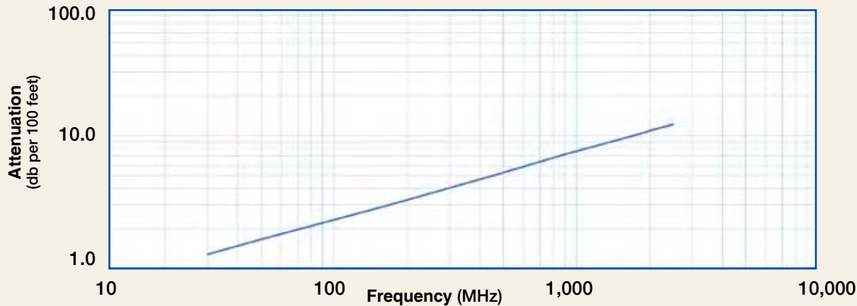
Attenuation vs. Frequency (typical)
