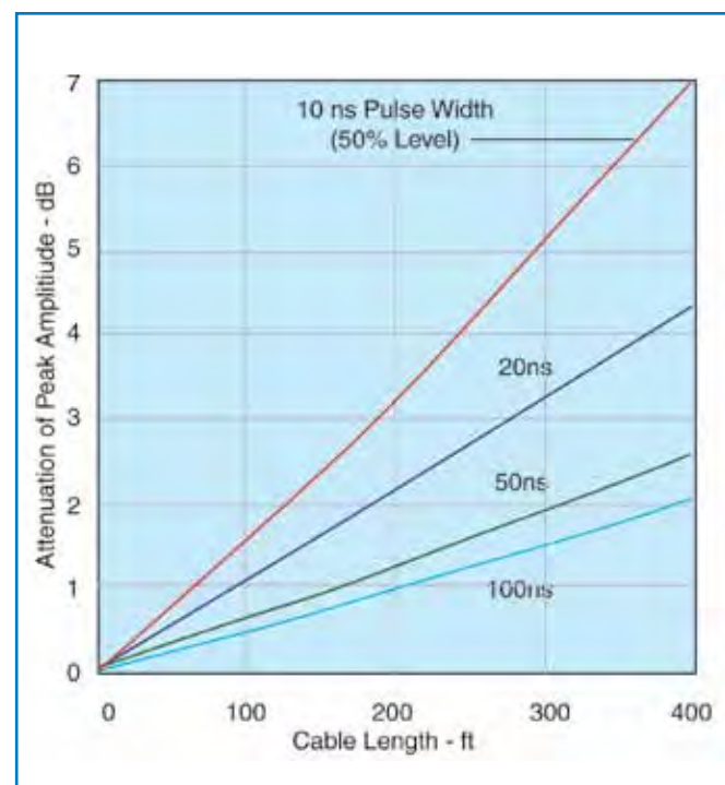
Fig. 12 Pulse Amplitude vs. Length
