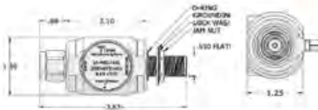
• LP-WBX-NMS 2000 - 6000MHz N Type M on Surge
