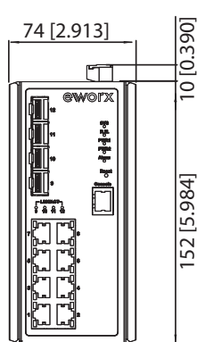
Model SE512-4SFP-T faceplate detail
