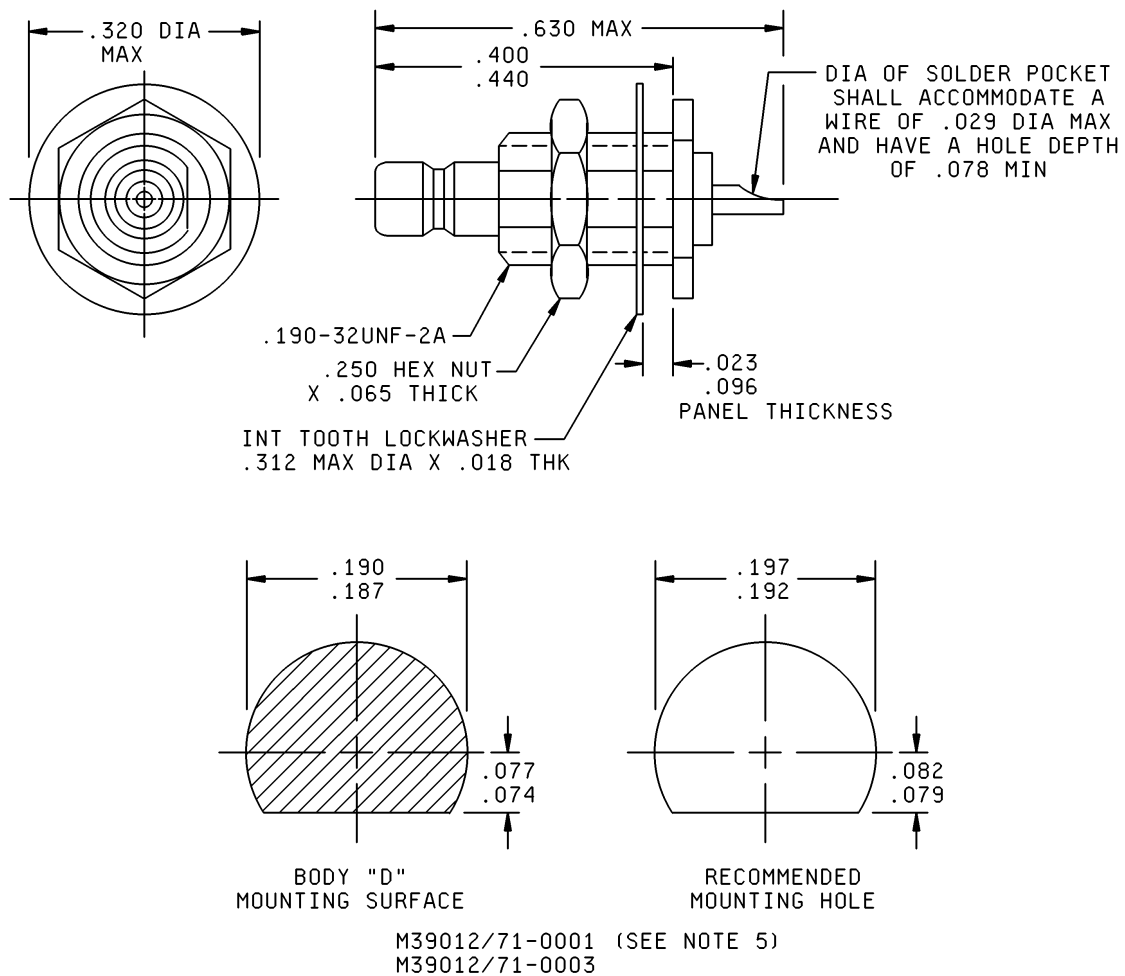
FIGURE 1. General configuration.
