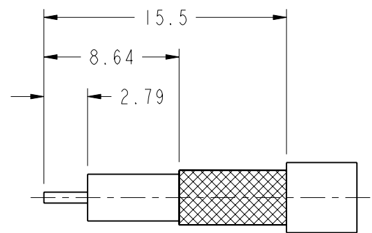
RECOMMENDED CABLE STRIPPING DIM'S SCALE 3.000
