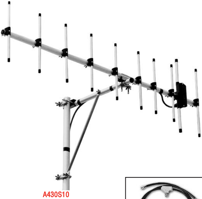
A430S10 (above) and A430S15 (right) are shown mounted with side mount bracket KB430.
