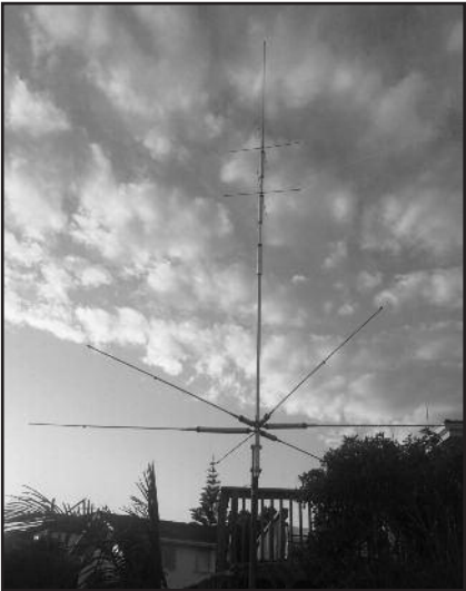
CP6AR Multiband Vertical Antenna Photo Courtesy: Ian Wilson, ZL10GX
