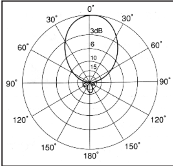
A502HB 51MHz Radiation Pattern
